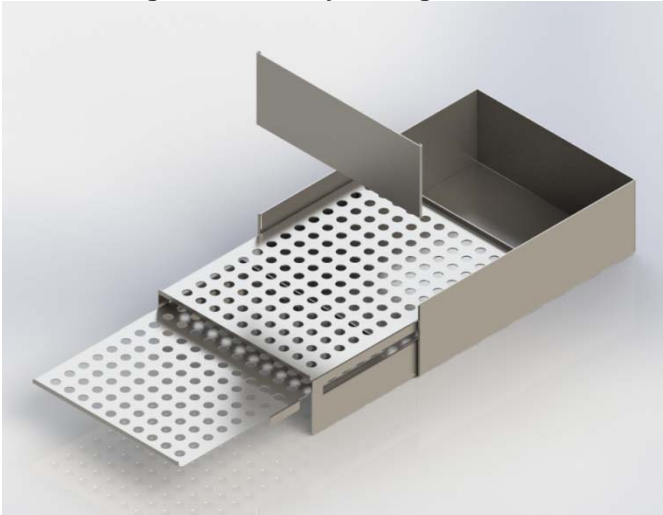
Quick dis-assembly of all parts for cleaning
